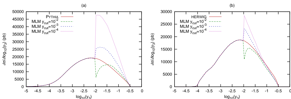
Figure 13: (a) The y_3 spectra at parton level for default PYTHIA and our PYTHIA implementation of the MLM algorithm for y_{MS} = 10^{-2} and for different values of the matrix element cutoff. (b) shows the same for HERWIG.
