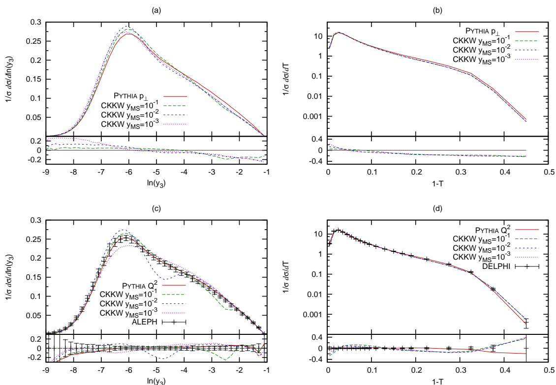
Figure 7: Charged plus neutral particle y_3 and charged particles thrust for our PYTHIA implementation of CKKW corrections with transverse momentum and virtuality ordered showers and using different merging scales. Figure (c) includes a comparison to ALEPH data and (d) a comparison to DELPHI data, where figure (a) and (b) only compare to the default PYTHIA, since the transverse momentum ordered shower has not yet been tuned to data.
