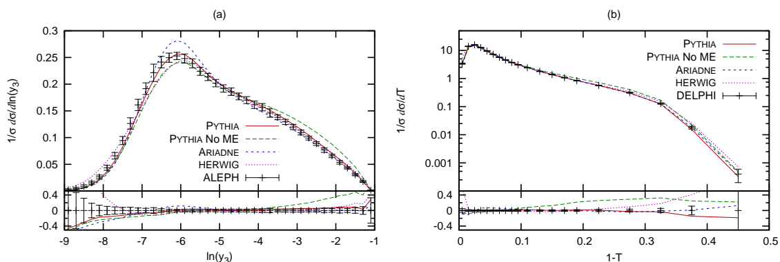
Figure 1: The y_3 spectra at parton level for PYTHIA, PYTHIA with matrix element reweighting switched off, ARIADNE and HERWIG.
