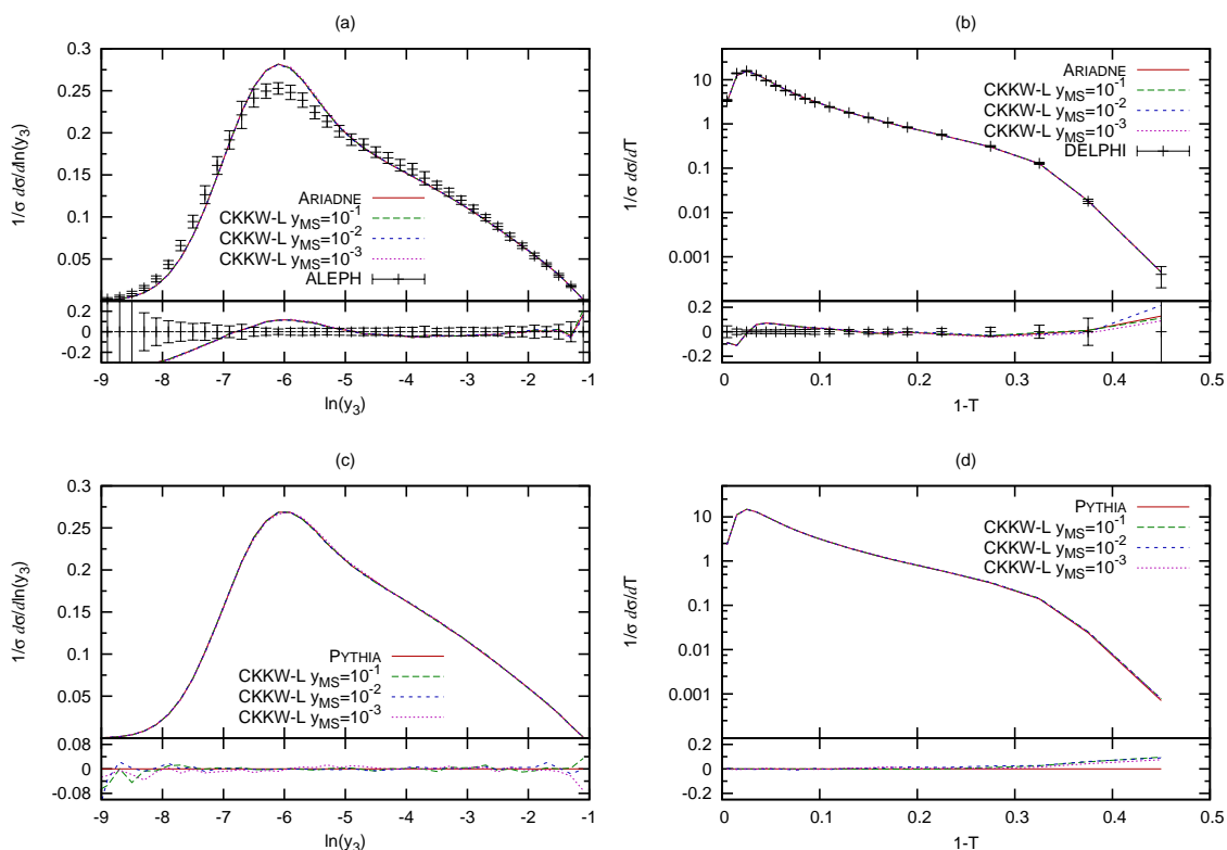
Figure 4: Charged plus neutral particle y_3 and charged particle thrust for the ARIADNE and PYTHIA implementation of CKKW-L corrections with different merging scales. Figure (a) includes a comparison to ALEPH data and (b) a comparison to DELPHI data, where figure (c) and (d) only compare to the default PYTHIA, since the p_{\perp} -ordered shower has not yet been tuned to data.
