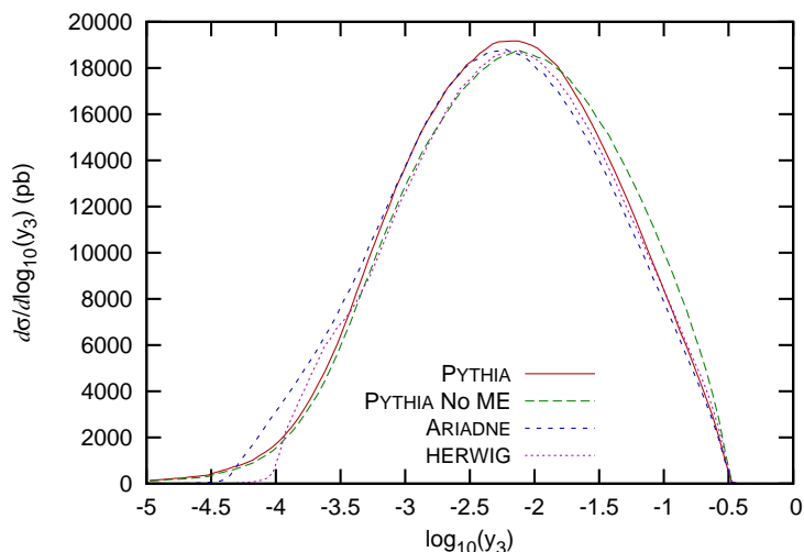
Figure 1: The y_3 spectra at parton level for PYTHIA, PYTHIA with matrix element reweighting switched off, ARIADNE and HERWIG.
