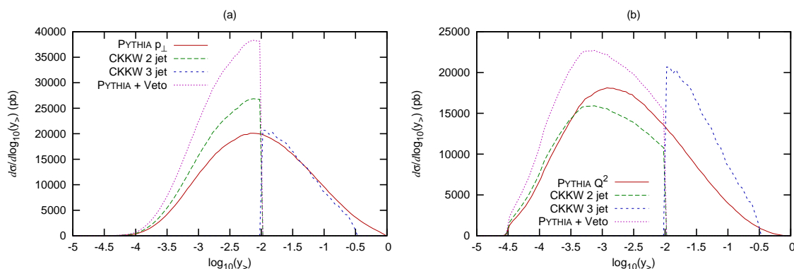
Figure 6: The maximum Durham k_{\perp} -value of any emission in the cascade for PYTHIA with p_{\perp} -ordered shower (and with the first order matrix element reweighting included) and for the two- and three-jet components in our PYTHIA implementation of CKKW corrections with a merging scale y_{MS} = 10^{-2} . An extra curve is included to show the two-jet contribution without the suppression from the analytic Sudakov form factor.
