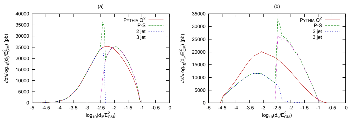
Figure 9: The Pseudo-Shower results, with \sqrt{d_{MS}} = 5 GeV and \delta = 1 GeV, split into two- and three-jet components compared to the default shower in PYTHIA (with first order matrix element reweighting included). (a) shows the d_3 distribution at parton level and (b) is the largest d -value of the emissions in the shower.
