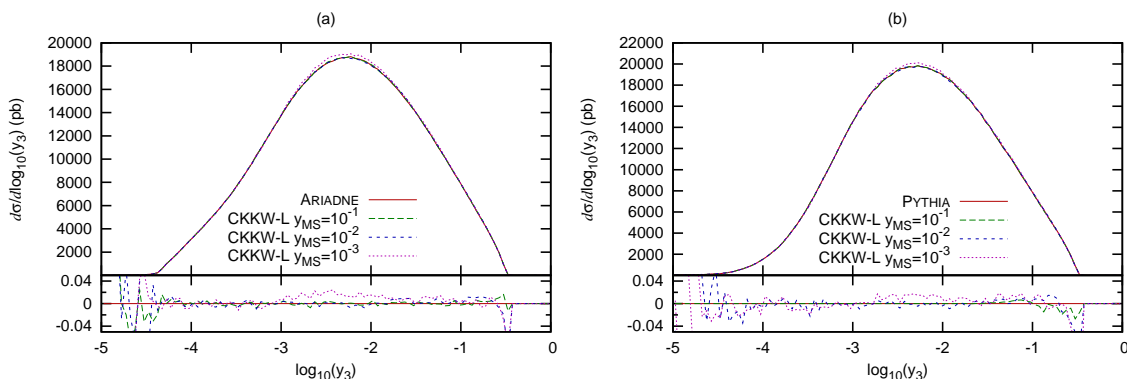
Figure 3: (a) The y_3 spectra at parton level for ARIADNE (the first order matrix element is included by construction) and for the ARIADNE implementation of CKKW-L corrections with different merging scales. (b) is the same for our PYTHIA implementation of CKKW-L corrections with different merging scales. The in-sets at the bottom of the plots show the relative differences between the CKKW-L results and the default shower, (\sigma_{\text{CKKW-L}} - \sigma_{\text{Shower}})/\sigma_{\text{Shower}} .
