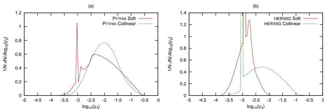
Figure 12: The y_3 spectra at parton level for PYTHIA (a) and HERWIG (b) when starting from a state with a soft or a collinear gluon with a merging scale of y = 10^{-3} and the scale in the Les Houches interface set to E_{CM} .
