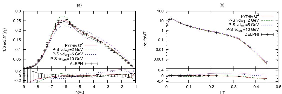
Figure 11: The charged plus neutral particle y_3 spectra (a) and charged particle thrust spectra (b) for PYTHIA (with first order matrix element reweighting included) and for our implementation of the Pseudo-Shower algorithms with different merging scales and \delta = 1 GeV compared to ALEPH and DELPHI data.
