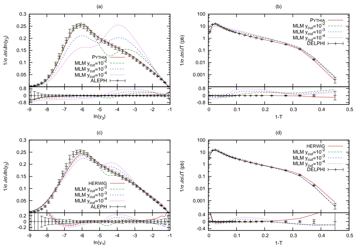
Figure 14: The charged plus neutral particle y_3 spectra (a) and the charged particle thrust spectra (b) for default PYTHIA and our PYTHIA implementation of the MLM algorithm for three different values of the matrix element cutoff. The HERWIG results are shown in (c) and (d) respectively.
